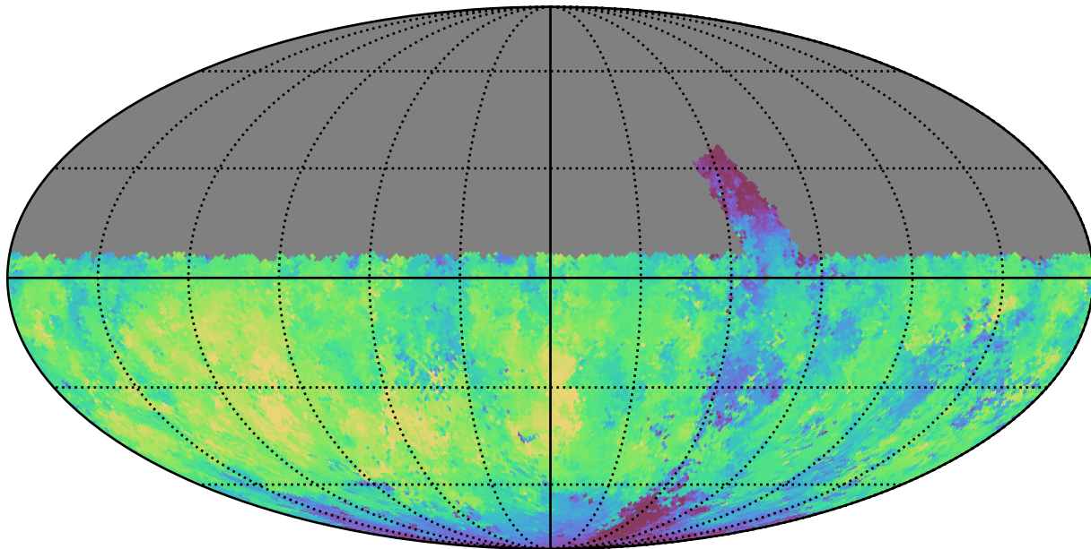
retro_baseline_v2.0_10yrs Yr 1 u band: Median fiveSigmaDepth
