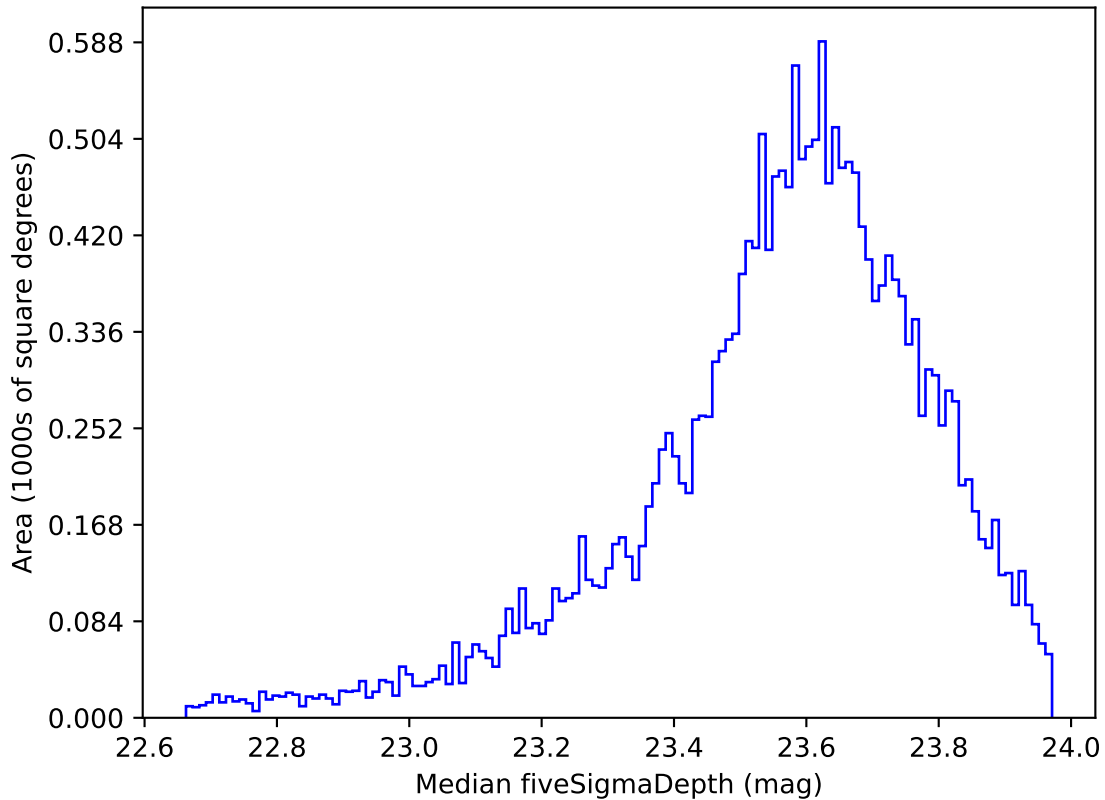
retro_baseline_v2.0_10yrs Yr 1 u band: Median fiveSigmaDepth
