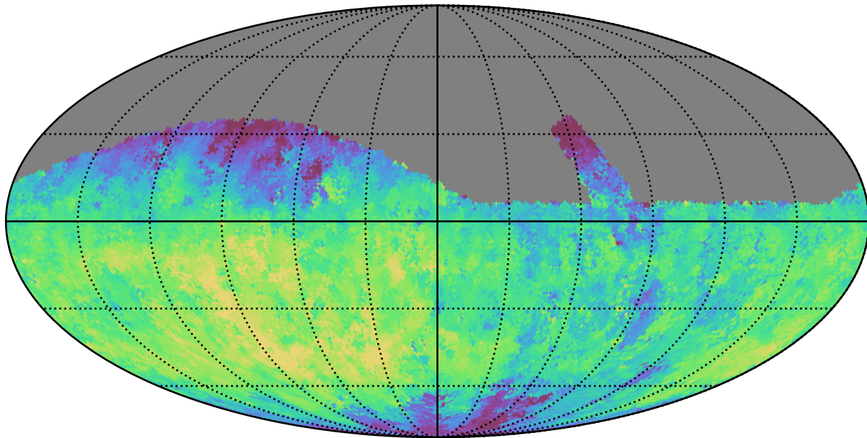
retro_baseline_v2.0_10yrs Yr 1 r band: Median fiveSigmaDepth
