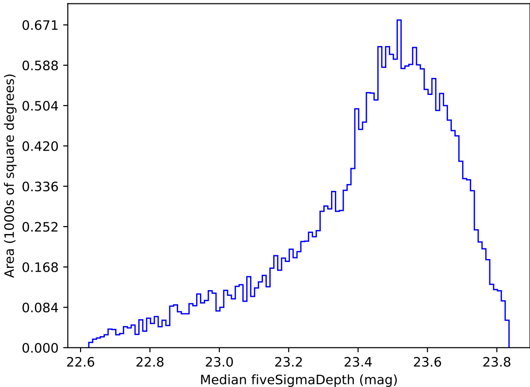
retro_baseline_v2.0_10yrs Yr 1 i band: Median fiveSigmaDepth
