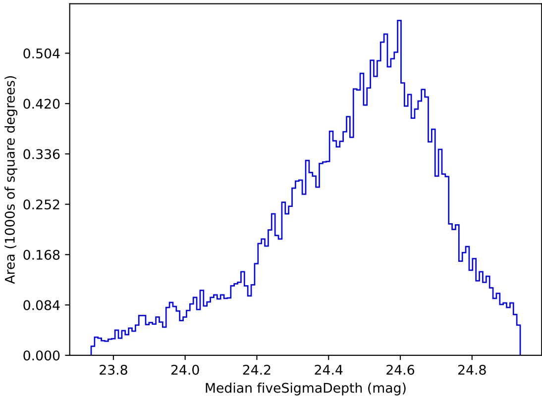
retro_baseline_v2.0_10yrs Yr 1 g band: Median fiveSigmaDepth
