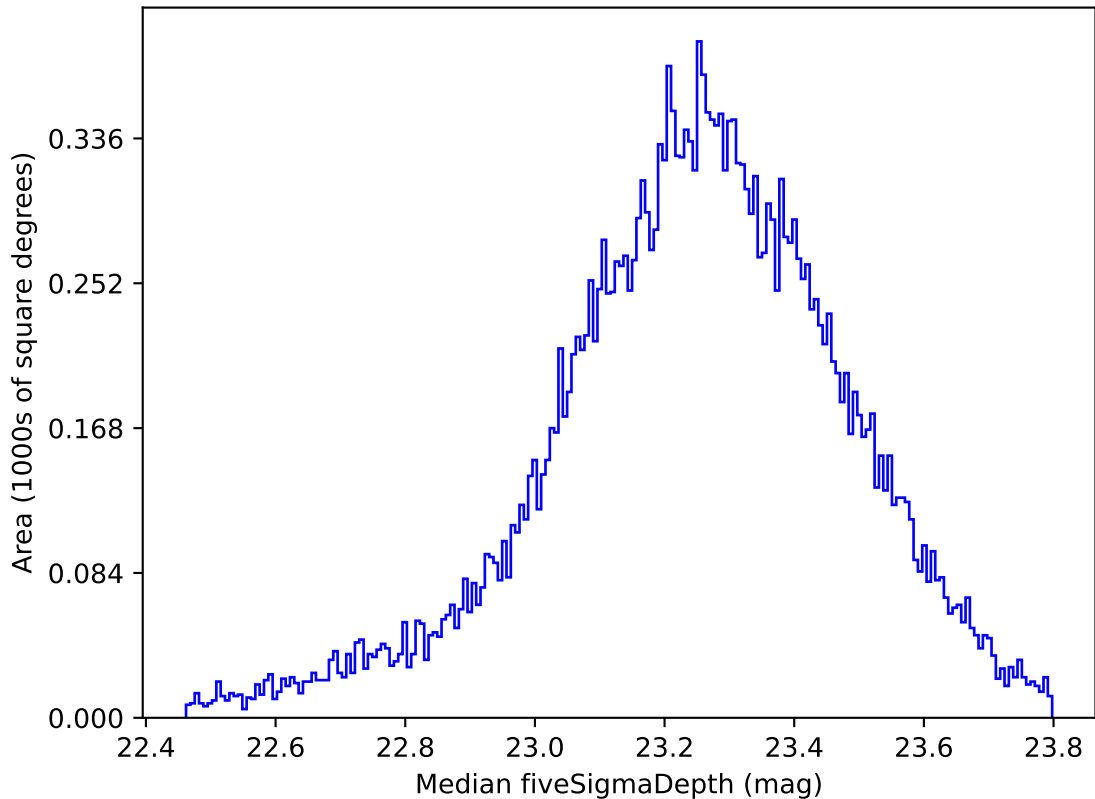
retro_baseline_v2.0_10yrs Yr 1 all bands: Median fiveSigmaDepth
