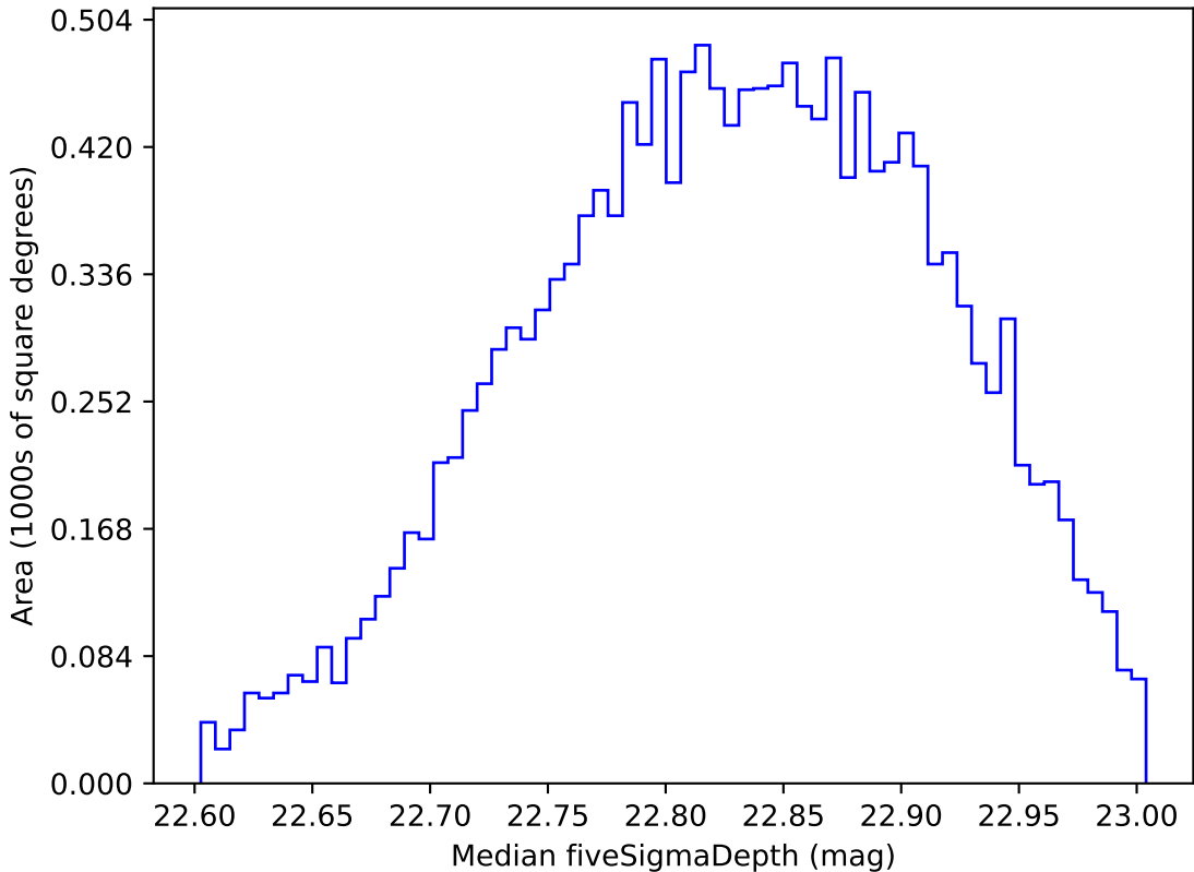
retro_baseline_v2.0_10yrs WFD z band: Median fiveSigmaDepth
