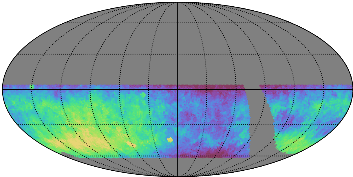
retro_baseline_v2.0_10yrs WFD y band: Median fiveSigmaDepth
