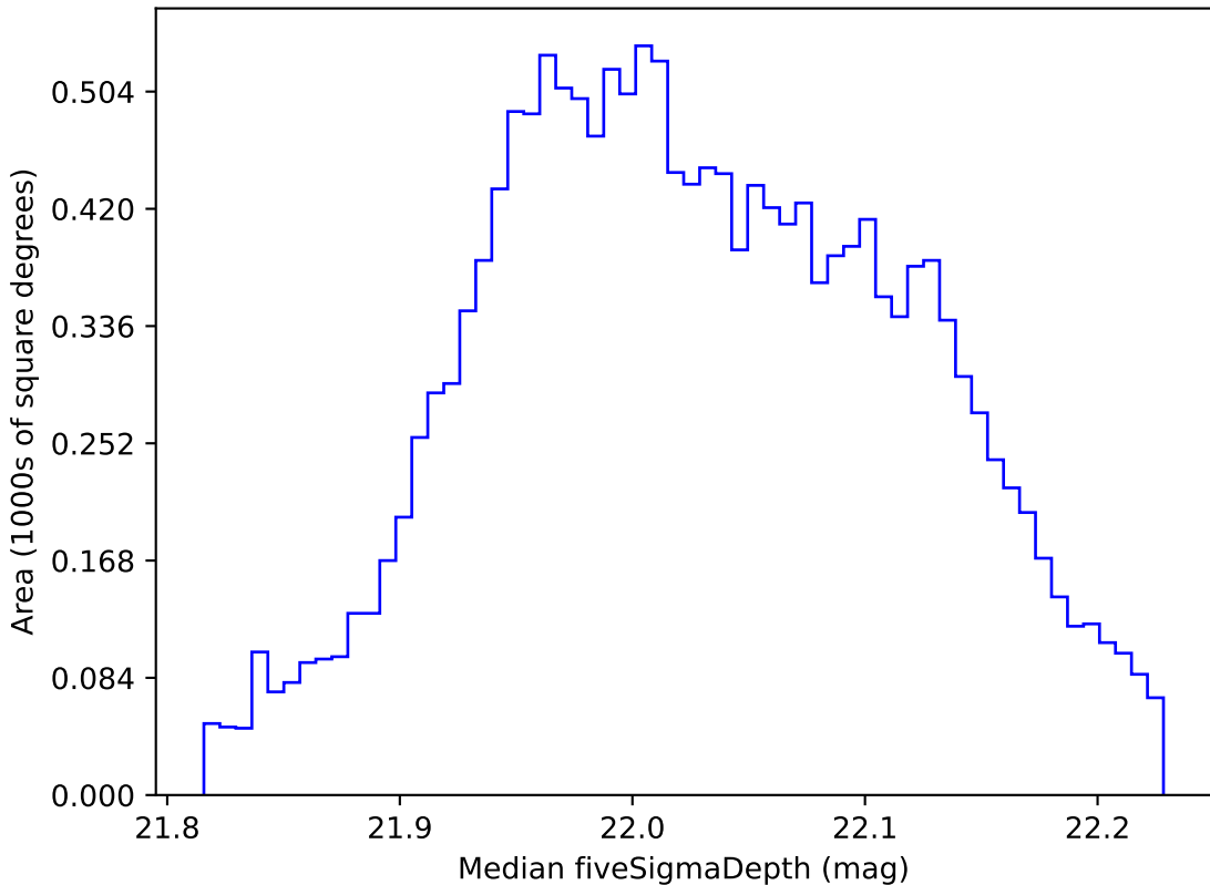
retro_baseline_v2.0_10yrs WFD y band: Median fiveSigmaDepth
