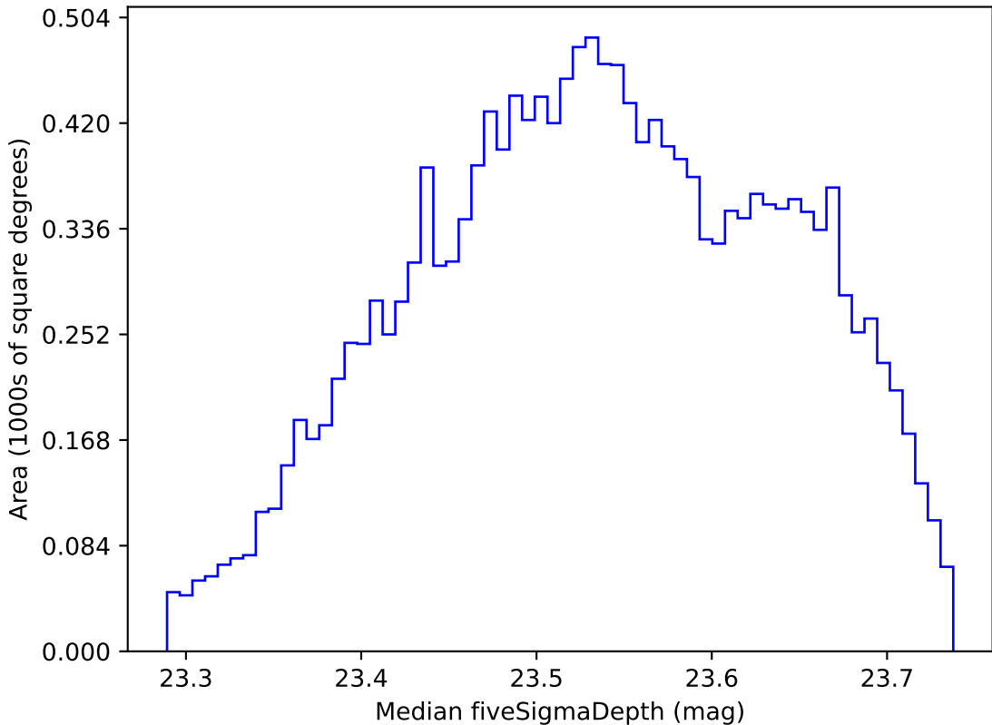
retro_baseline_v2.0_10yrs WFD u band: Median fiveSigmaDepth
