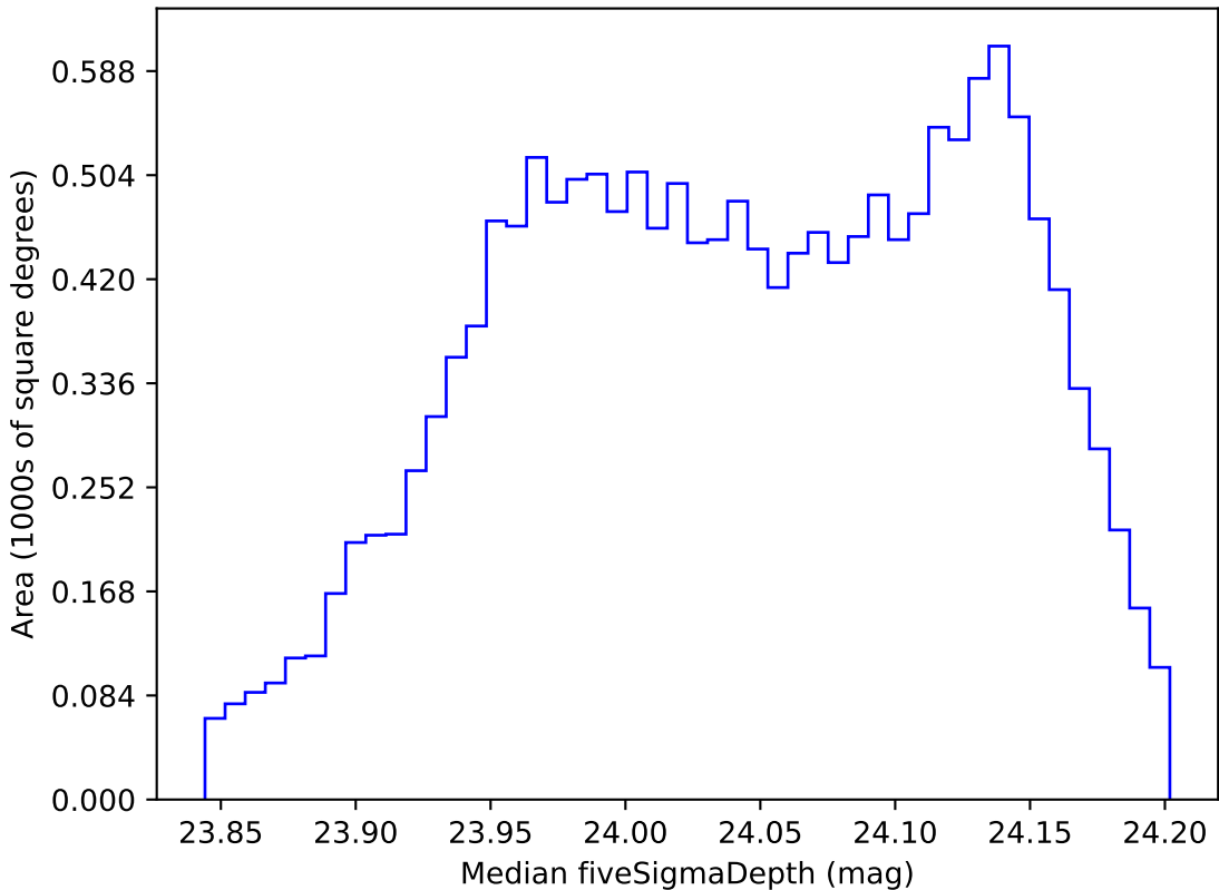
retro_baseline_v2.0_10yrs WFD r band: Median fiveSigmaDepth
