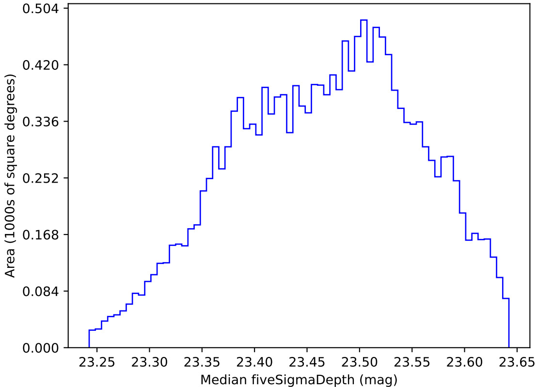
retro_baseline_v2.0_10yrs WFD i band: Median fiveSigmaDepth
