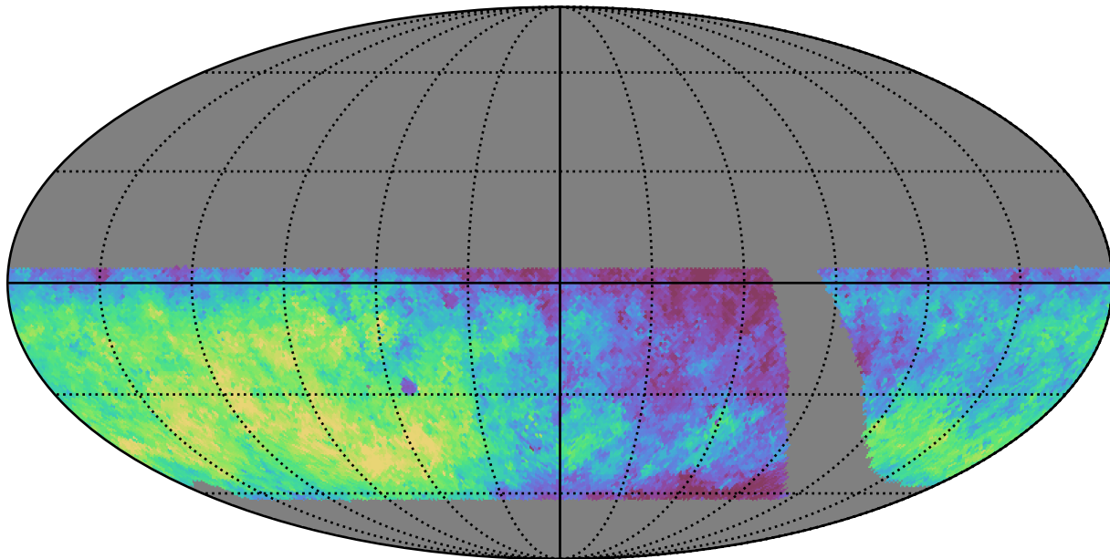
retro_baseline_v2.0_10yrs WFD g band: Median fiveSigmaDepth
