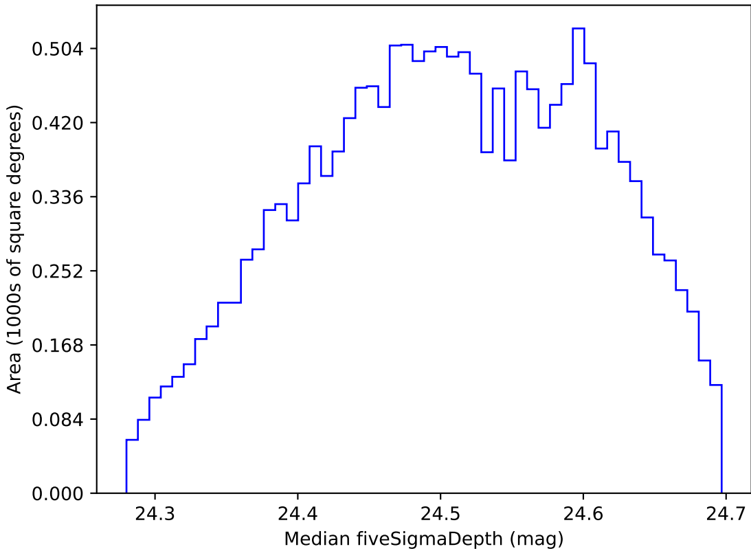
retro_baseline_v2.0_10yrs WFD g band: Median fiveSigmaDepth
