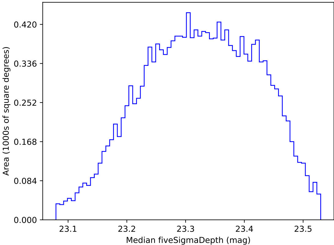
retro_baseline_v2.0_10yrs WFD all bands: Median fiveSigmaDepth
