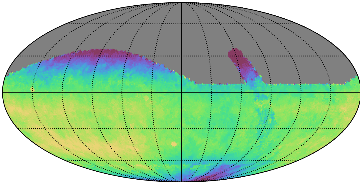
retro_baseline_v2.0_10yrs All sky z band: Median fiveSigmaDepth
