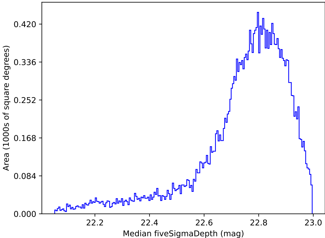
retro_baseline_v2.0_10yrs All sky z band: Median fiveSigmaDepth
