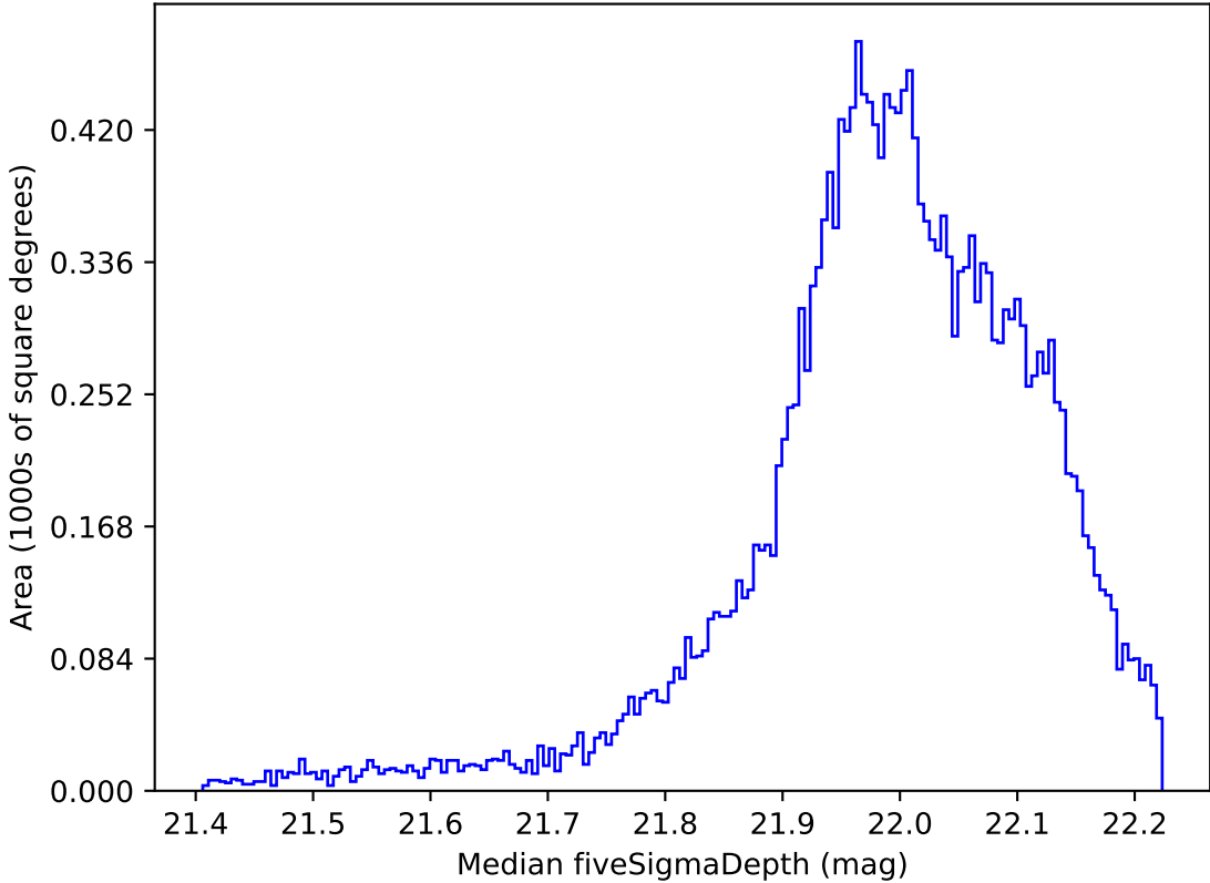
retro_baseline_v2.0_10yrs All sky y band: Median fiveSigmaDepth
