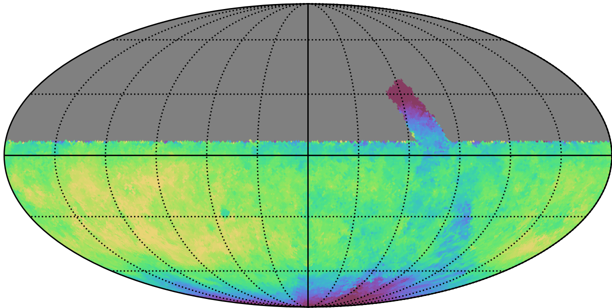
retro_baseline_v2.0_10yrs All sky u band: Median fiveSigmaDepth
