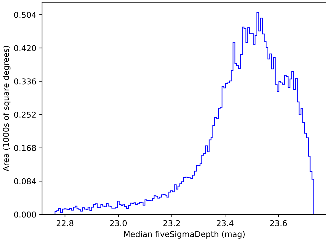
retro_baseline_v2.0_10yrs All sky u band: Median fiveSigmaDepth
