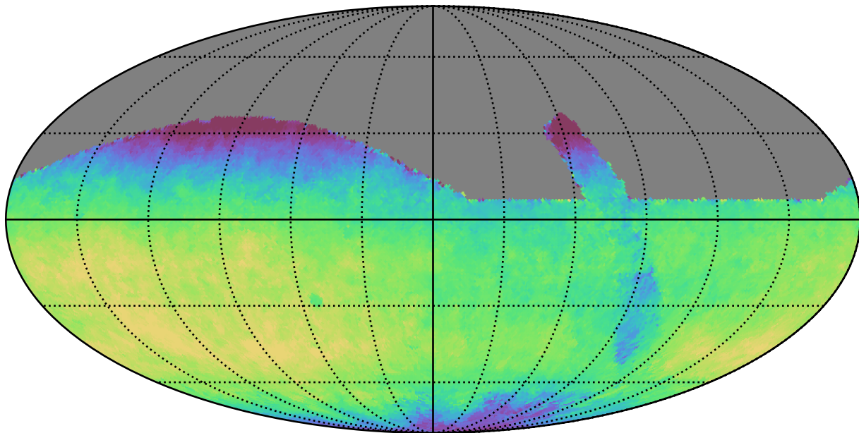
retro_baseline_v2.0_10yrs All sky r band: Median fiveSigmaDepth
