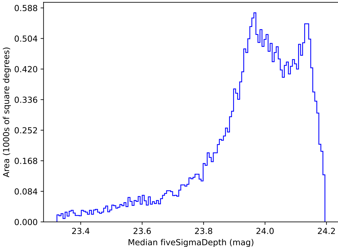
retro_baseline_v2.0_10yrs All sky r band: Median fiveSigmaDepth
