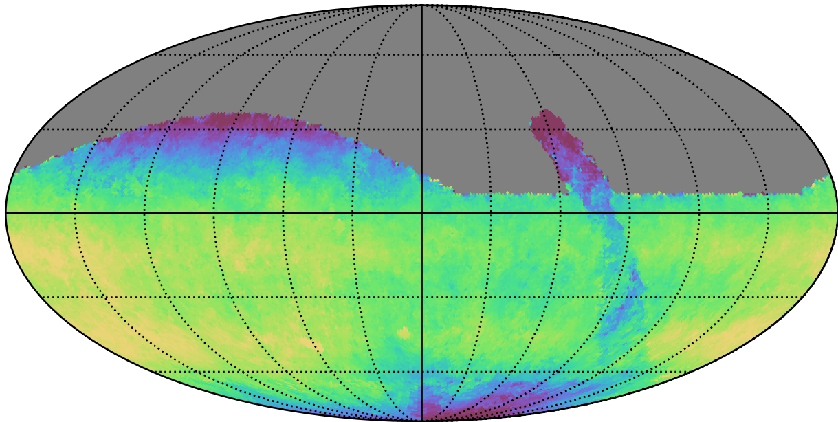
retro_baseline_v2.0_10yrs All sky i band: Median fiveSigmaDepth
