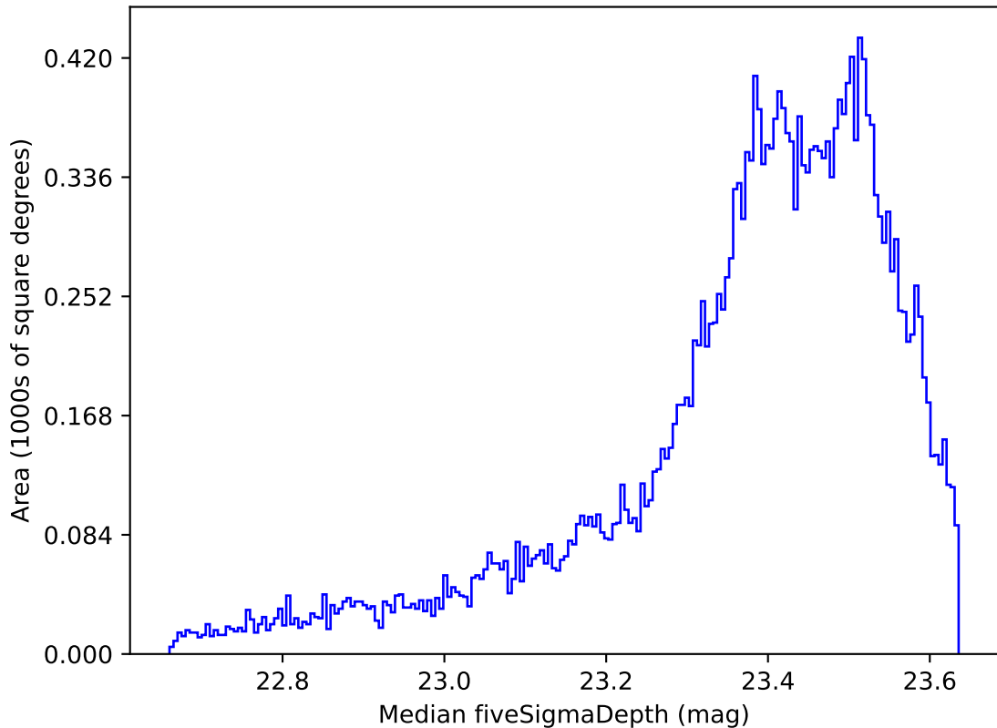
retro_baseline_v2.0_10yrs All sky i band: Median fiveSigmaDepth
