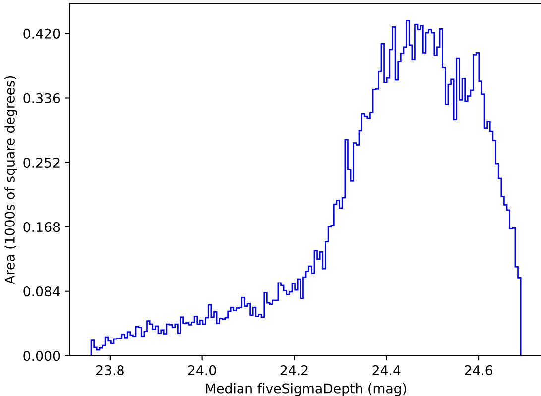
retro_baseline_v2.0_10yrs All sky g band: Median fiveSigmaDepth
