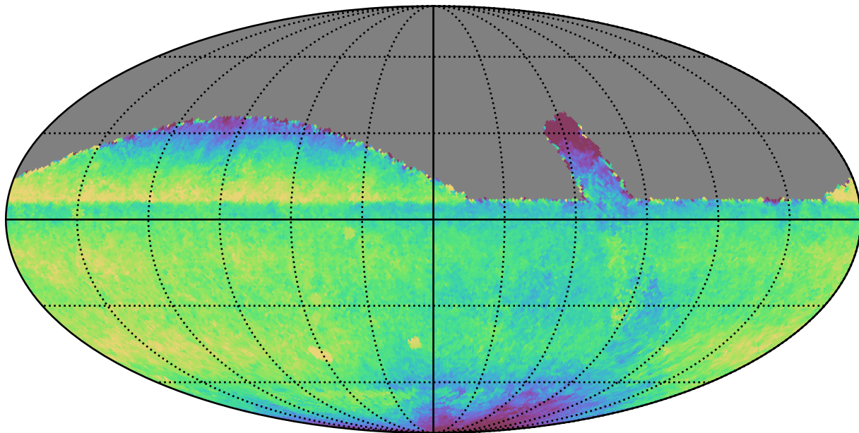
retro_baseline_v2.0_10yrs All sky all bands: Median fiveSigmaDepth
