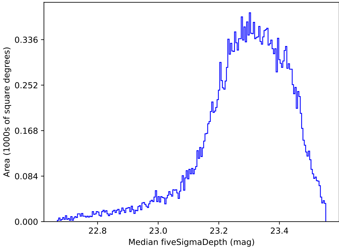
retro_baseline_v2.0_10yrs All sky all bands: Median fiveSigmaDepth
