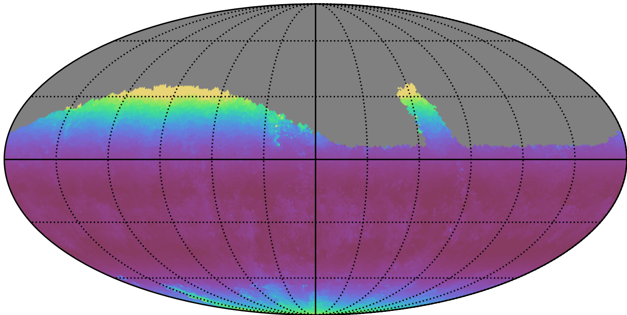
retro_baseline_v2.0_10yrs Yr 1 z band: Median airmass
