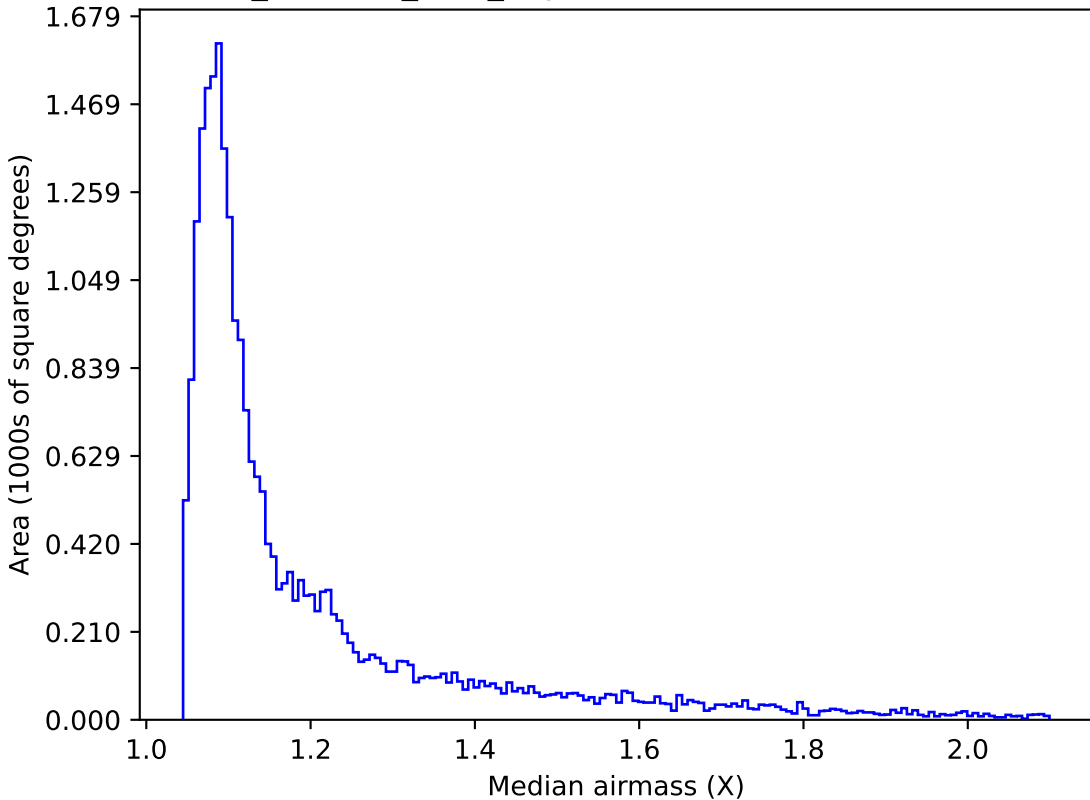
retro_baseline_v2.0_10yrs Yr 1 z band: Median airmass
