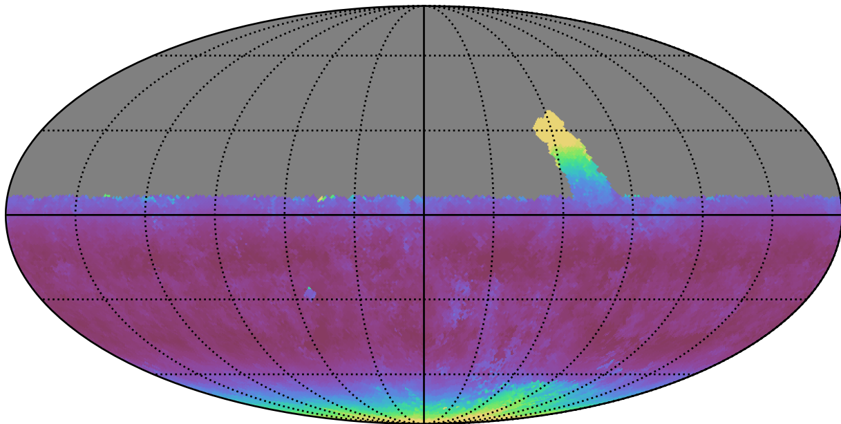
retro_baseline_v2.0_10yrs Yr 1 y band: Median airmass
