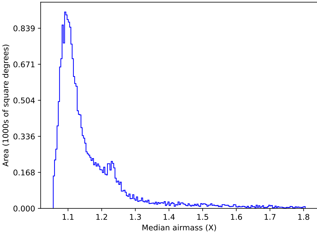
retro_baseline_v2.0_10yrs Yr 1 y band: Median airmass
