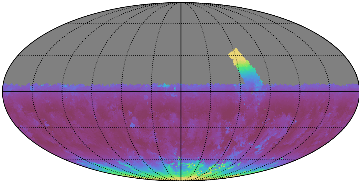
retro_baseline_v2.0_10yrs Yr 1 u band: Median airmass
