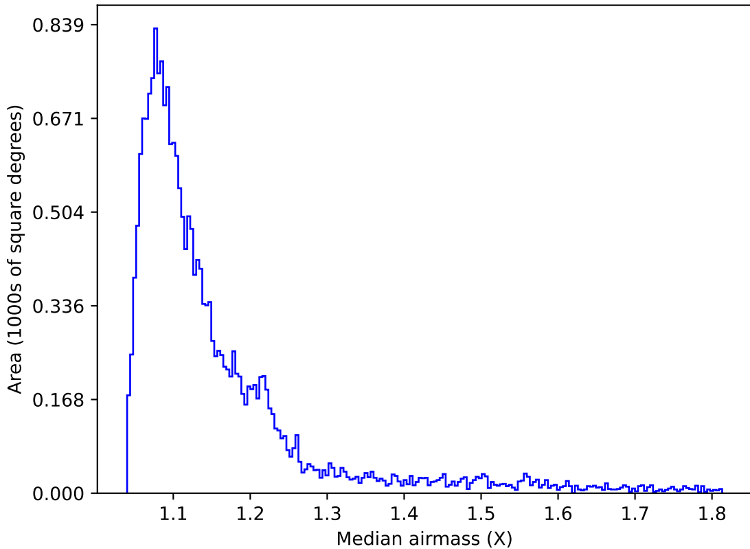
retro_baseline_v2.0_10yrs Yr 1 u band: Median airmass
