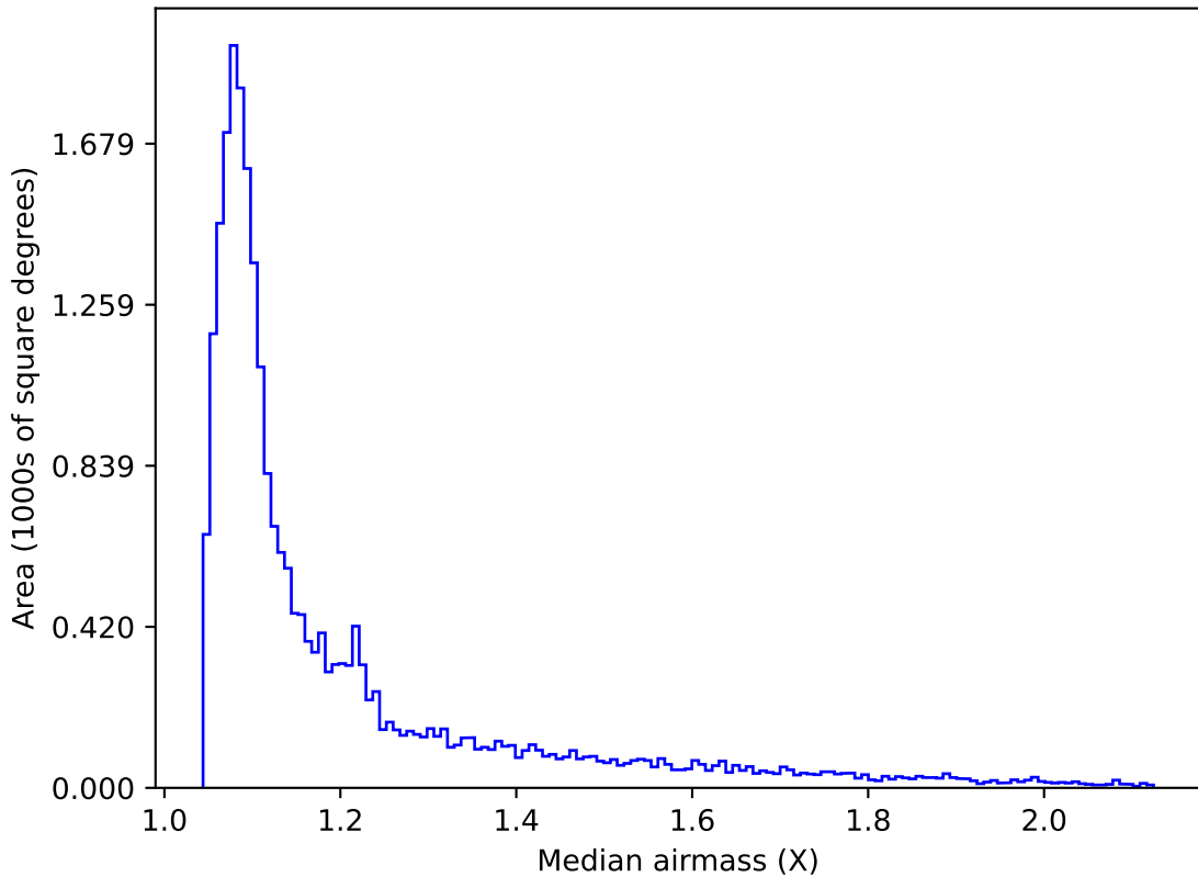
retro_baseline_v2.0_10yrs Yr 1 r band: Median airmass
