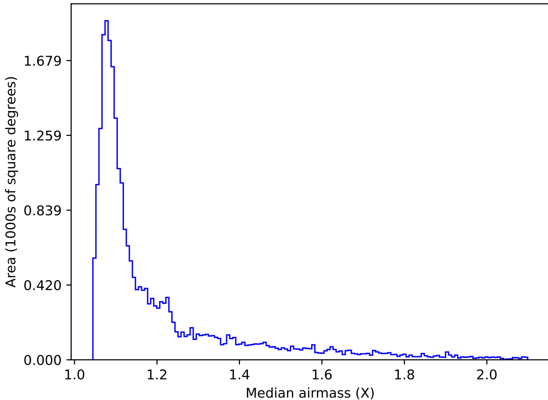
retro_baseline_v2.0_10yrs Yr 1 i band: Median airmass
