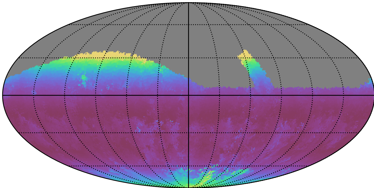
retro_baseline_v2.0_10yrs Yr 1 g band: Median airmass
