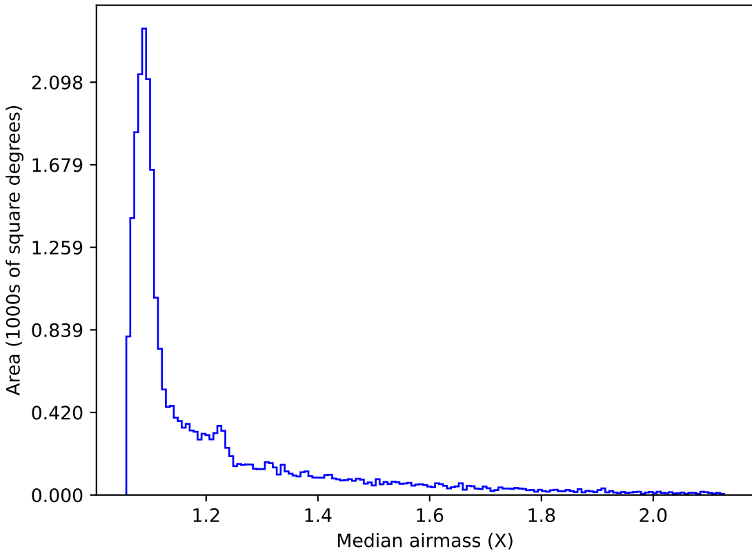
retro_baseline_v2.0_10yrs Yr 1 all bands: Median airmass
