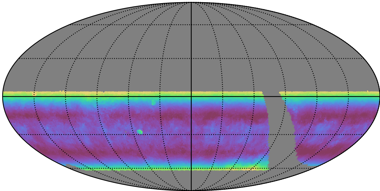
retro_baseline_v2.0_10yrs WFD z band: Median airmass
