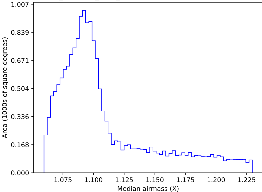
retro_baseline_v2.0_10yrs WFD z band: Median airmass
