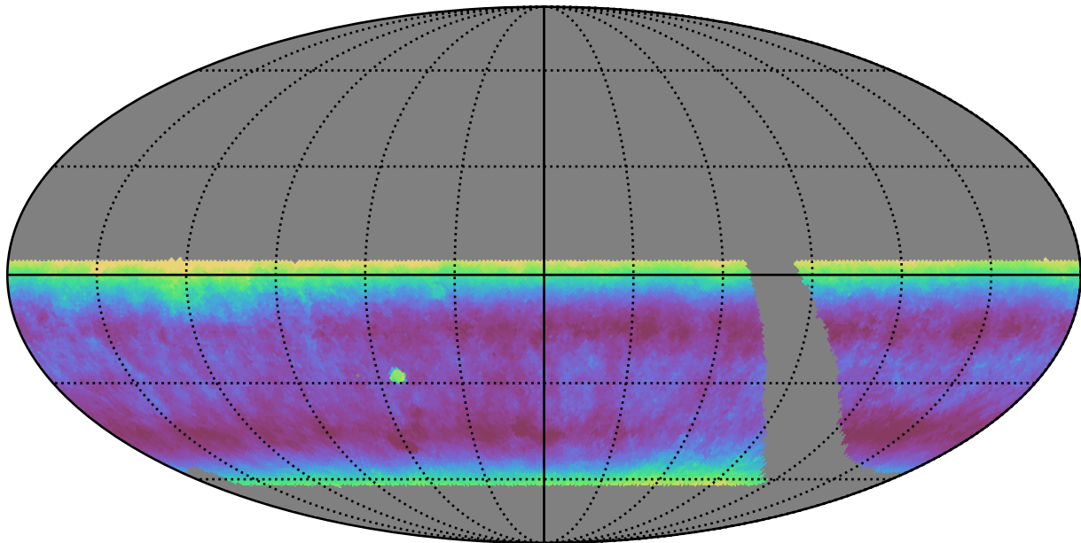
retro_baseline_v2.0_10yrs WFD y band: Median airmass
