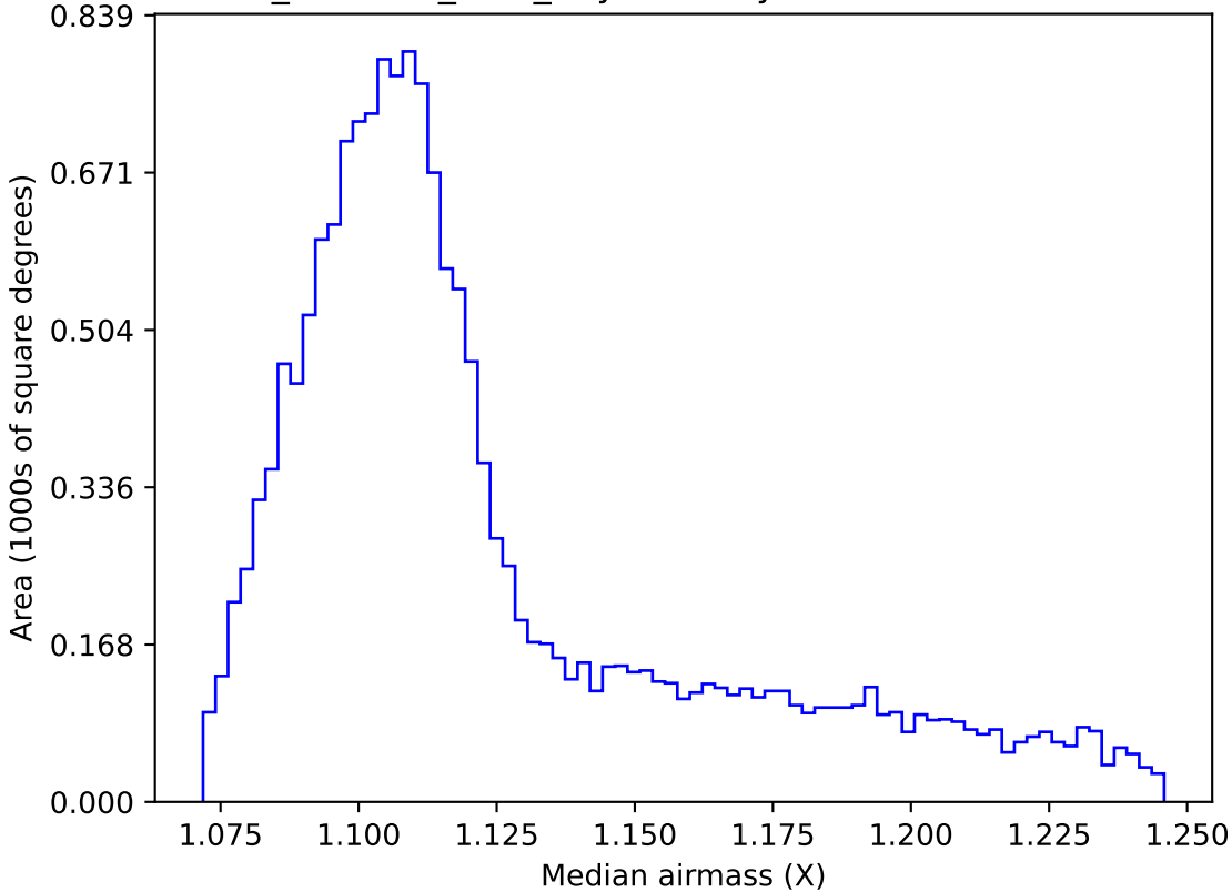
retro_baseline_v2.0_10yrs WFD y band: Median airmass
