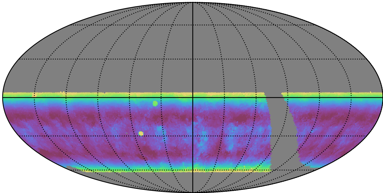
retro_baseline_v2.0_10yrs WFD u band: Median airmass
