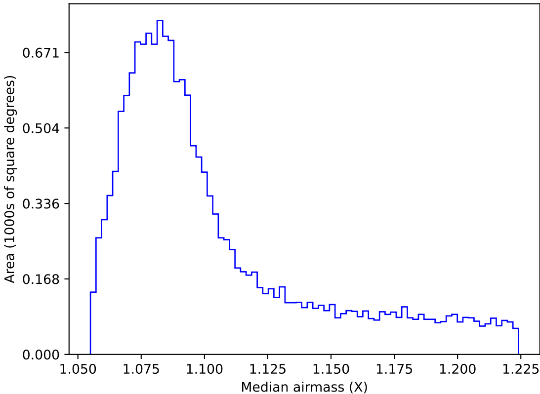
retro_baseline_v2.0_10yrs WFD u band: Median airmass
