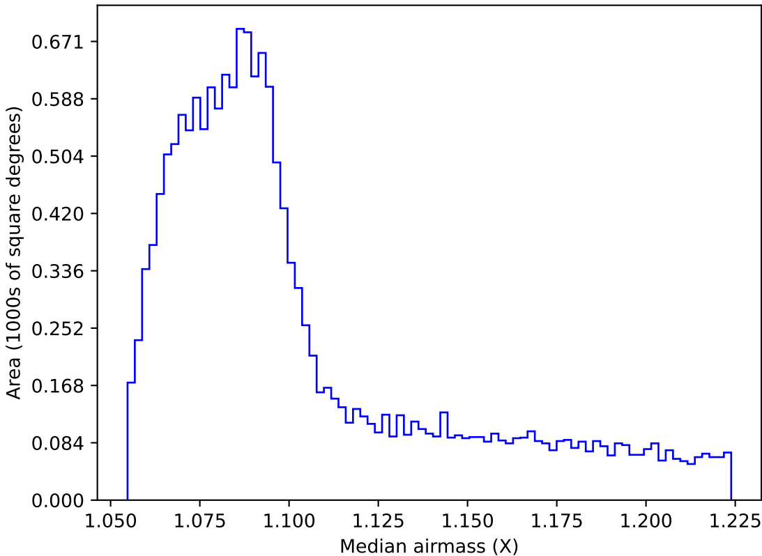
retro_baseline_v2.0_10yrs WFD i band: Median airmass
