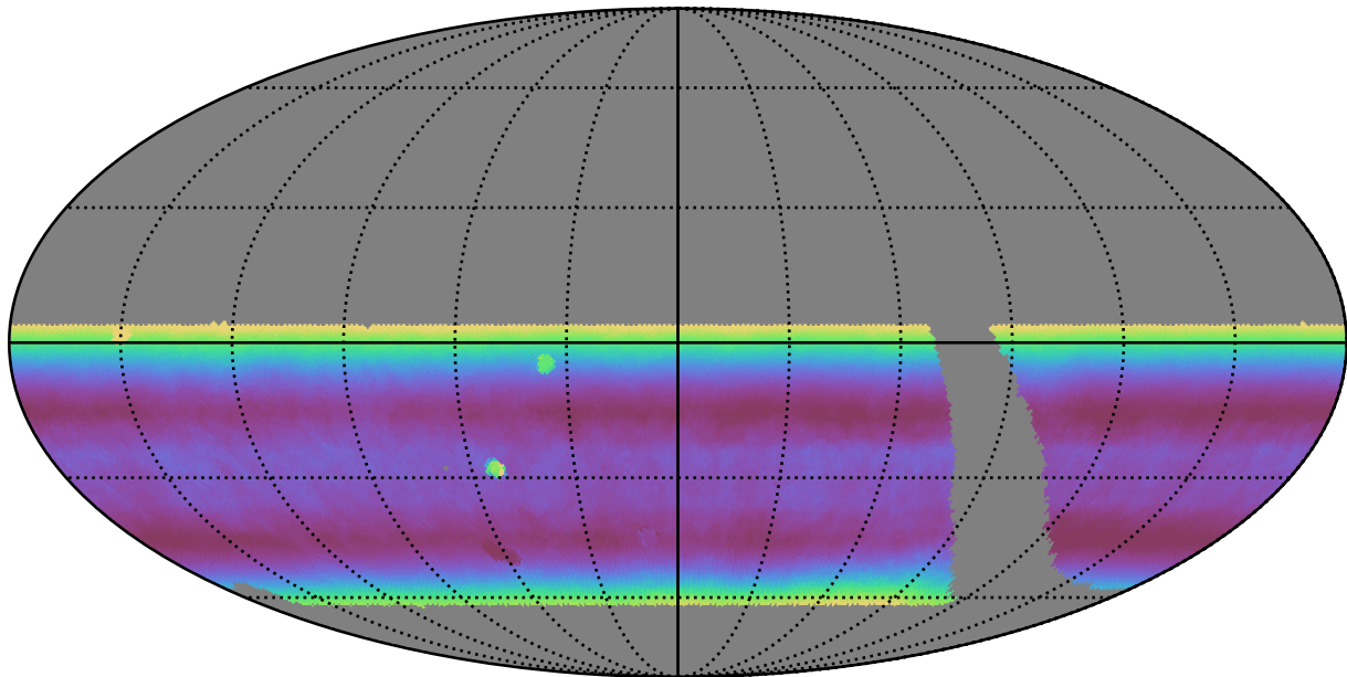
retro_baseline_v2.0_10yrs WFD all bands: Median airmass
