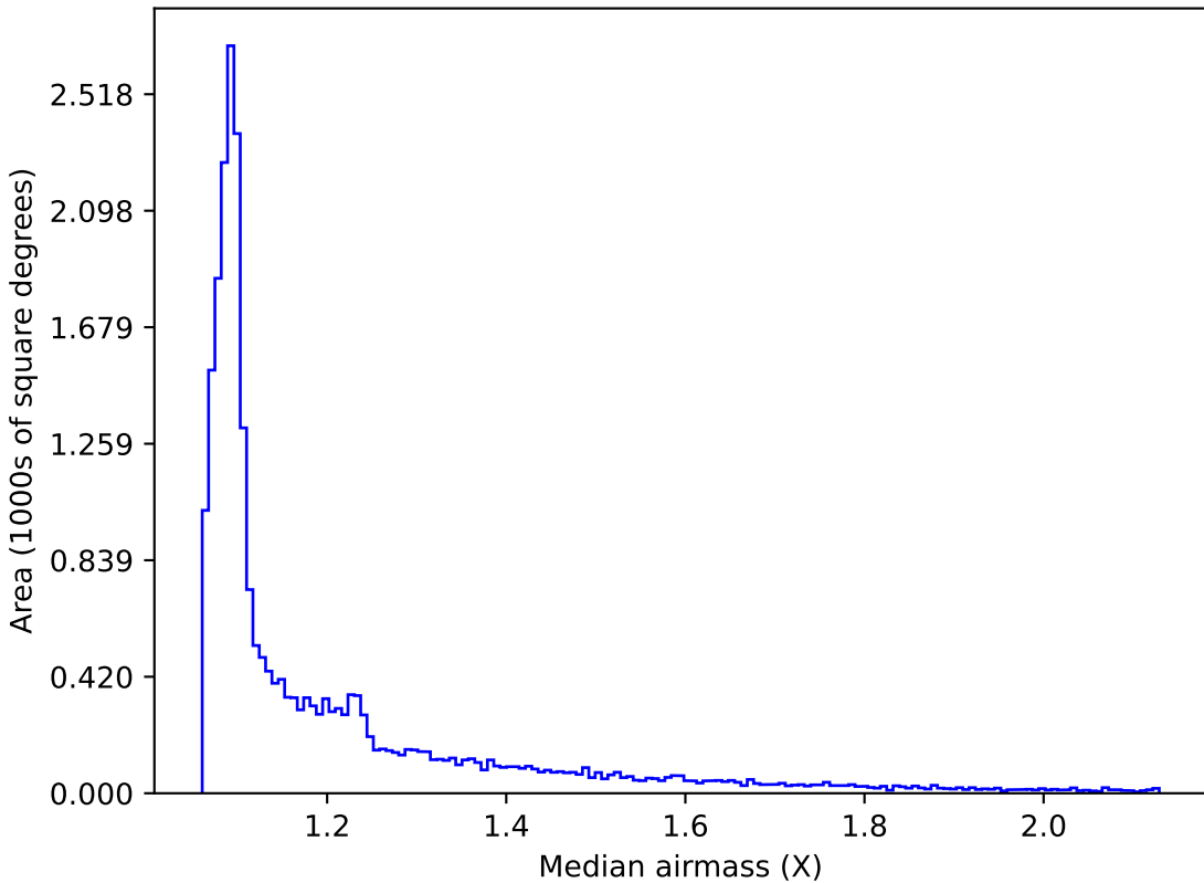
retro_baseline_v2.0_10yrs All sky z band: Median airmass
