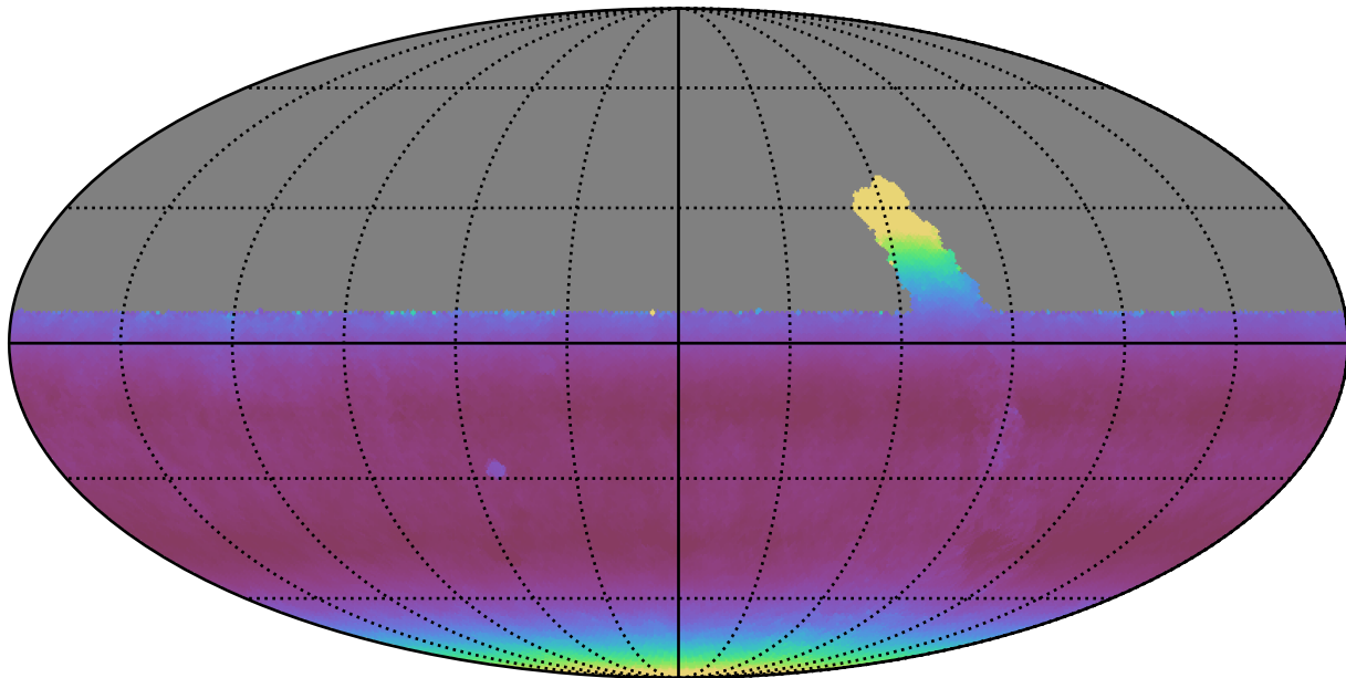
retro_baseline_v2.0_10yrs All sky y band: Median airmass
