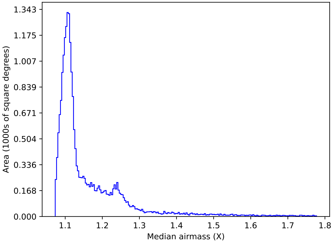
retro_baseline_v2.0_10yrs All sky y band: Median airmass
