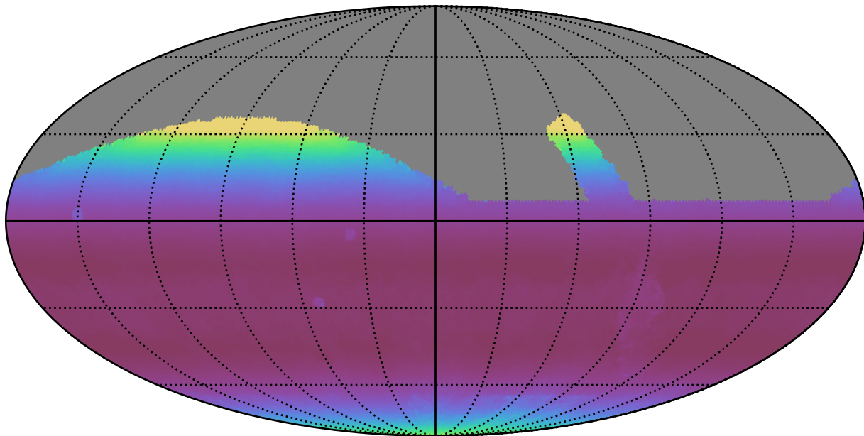
retro_baseline_v2.0_10yrs All sky r band: Median airmass
