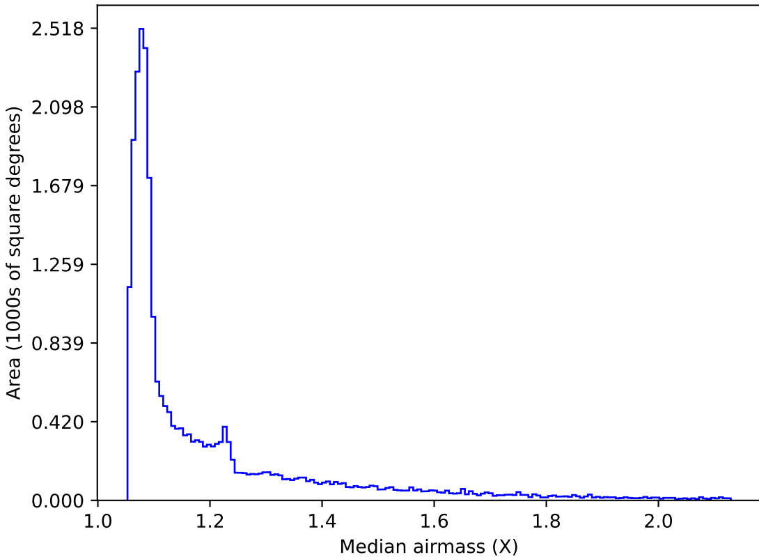
retro_baseline_v2.0_10yrs All sky r band: Median airmass
